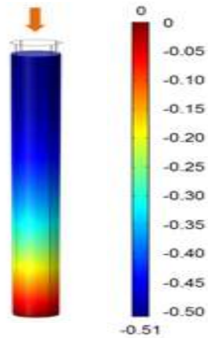
[Fig. 3] Distribution of piezopotential along a ZnO nanorod under axial strain calculated by finite element method. The growth direction of the nanorod is along the c-axis. L=600nm, d=60nm from [6]. (Copyright 2016 Journal of Visualized Experiments)
