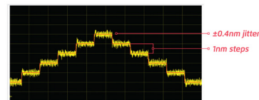
NanoPWM™
